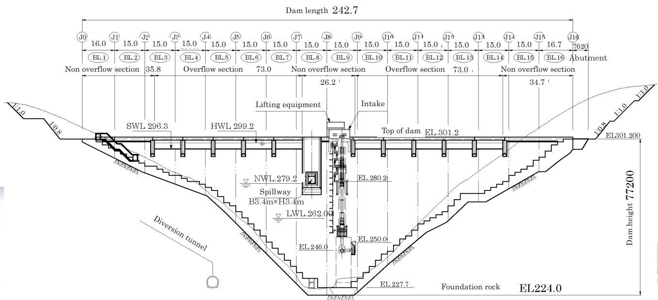
Figure-3 Upstream face
