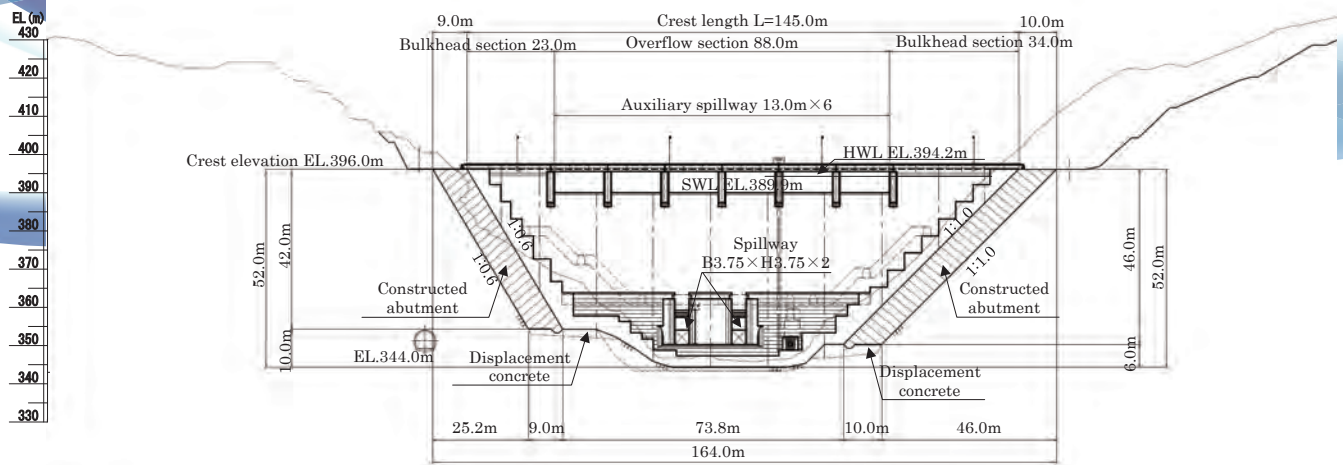
Figure-2 Up stream face
