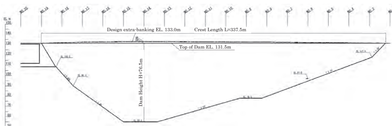
Figure-3 Longitudinal Profile
