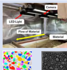
Image Granularity Monitoring Rapid determination of particle size distribution of geomaterials by digital camera image analysis
