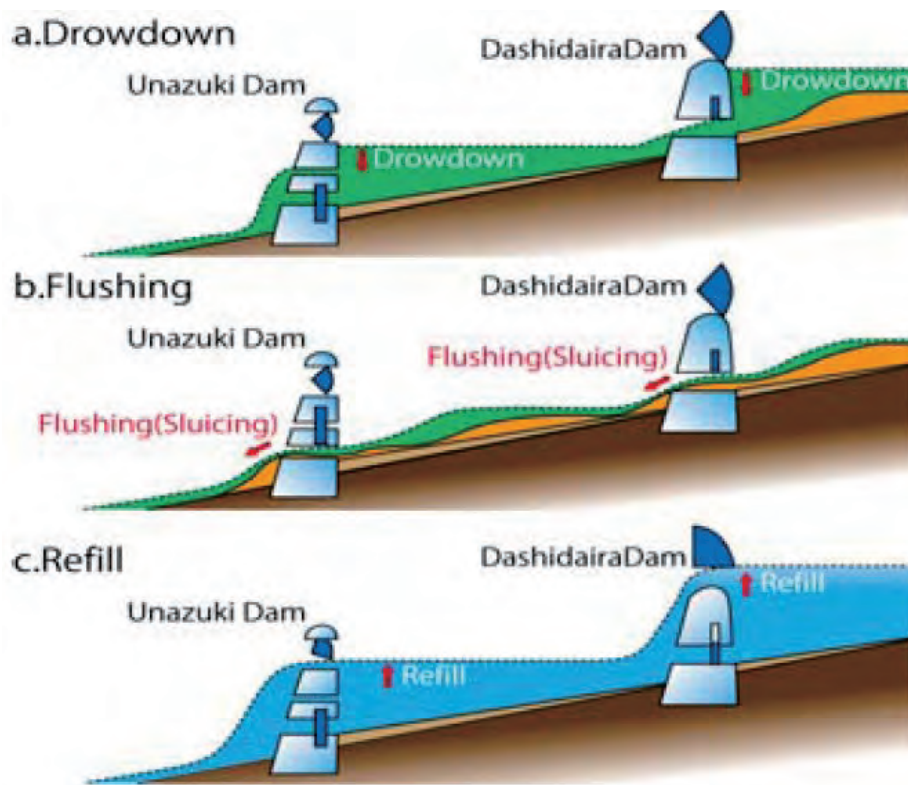
Fig. 4 Coordinated Sediment Flushing in the Kurobe River
