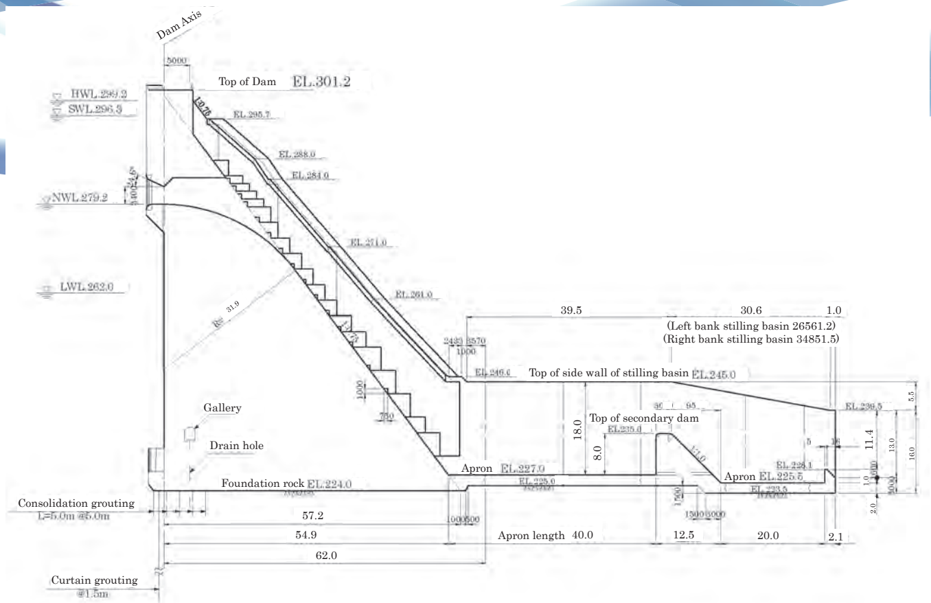
Figure-2 Typical section
